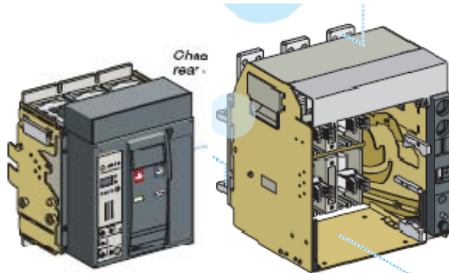
ACB : Withdrawable Type
